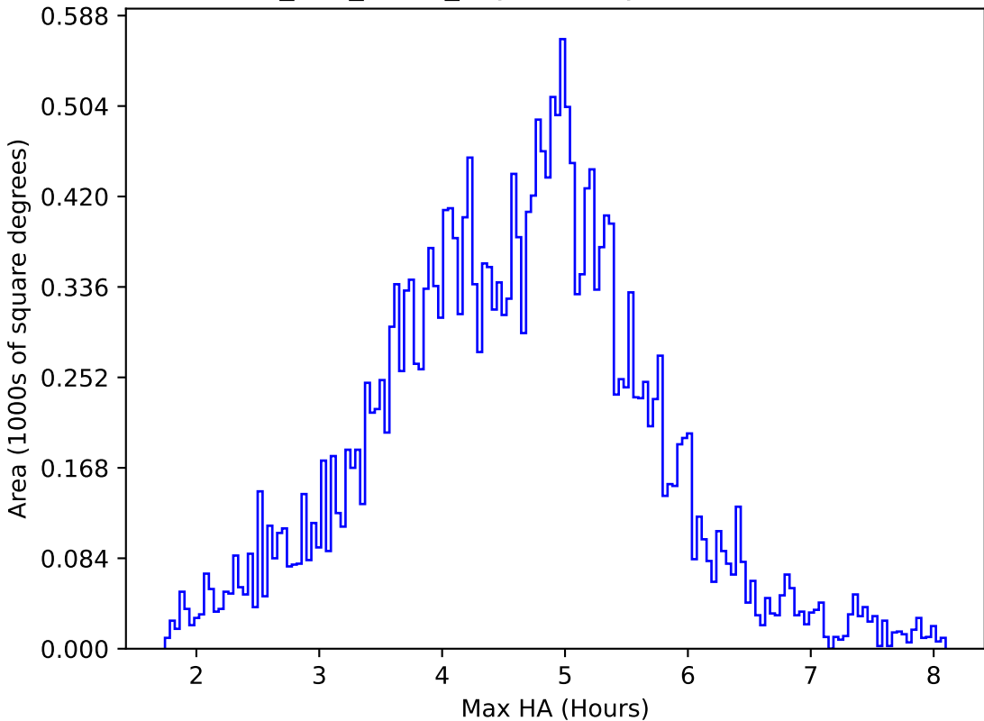
too_100_4v3.4_10yrs All sky z band: Max HA
