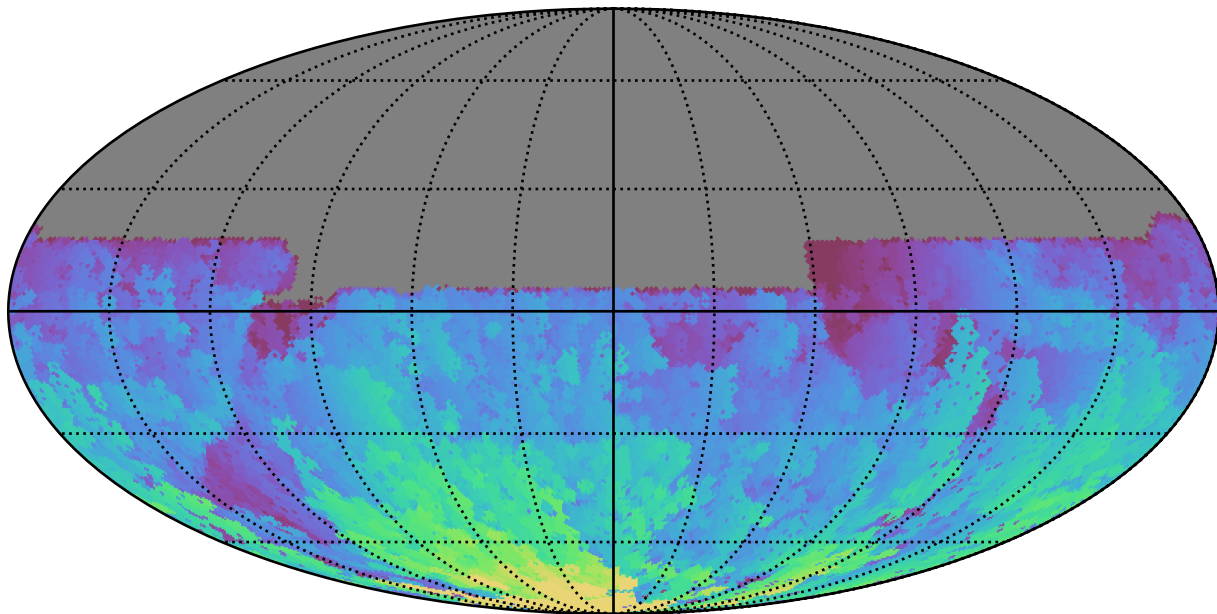
too_100_4v3.4_10yrs All sky u band: Max HA
