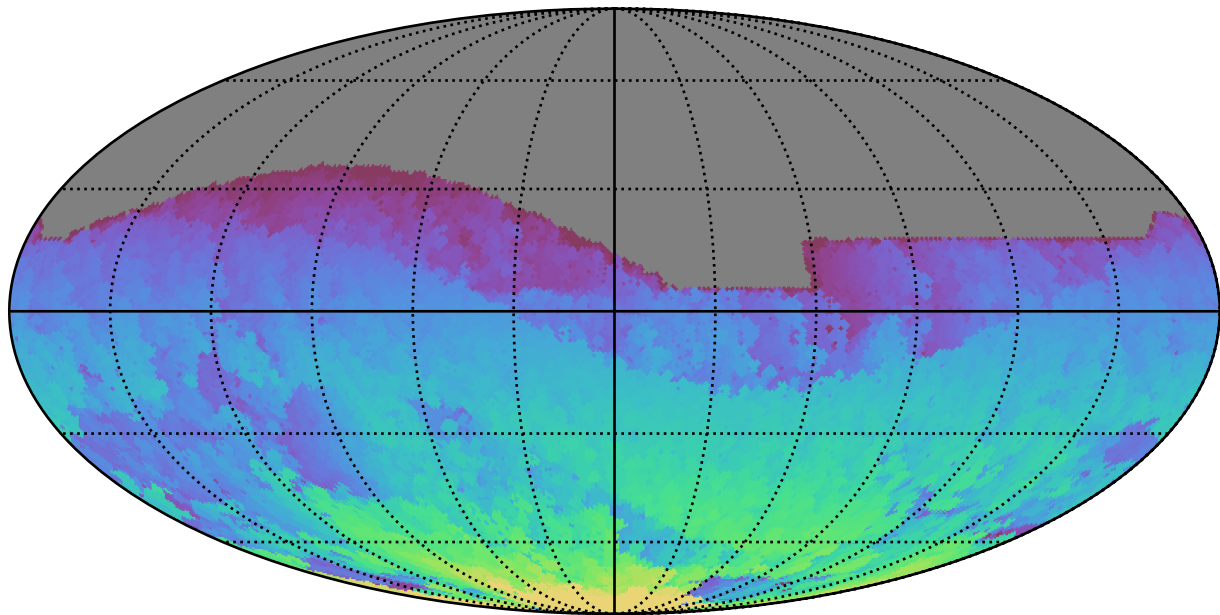
too_100_4v3.4_10yrs All sky i band: Max HA
