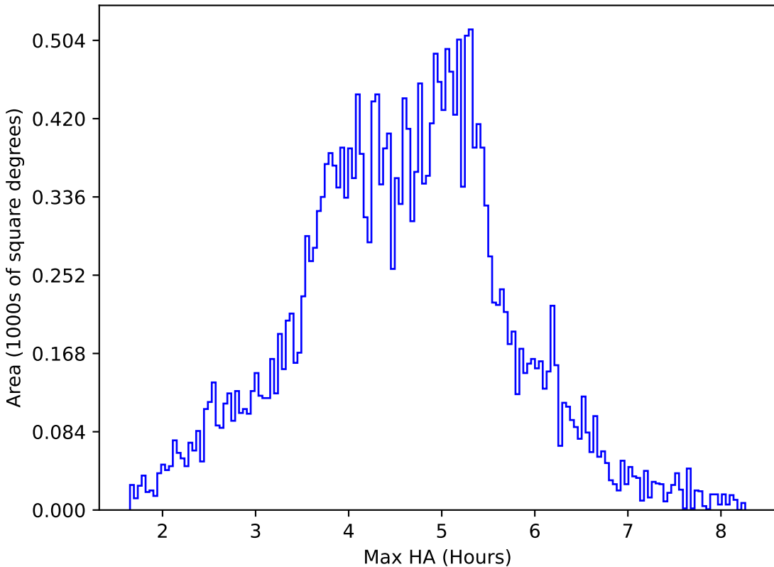
too_100_4v3.4_10yrs All sky i band: Max HA
