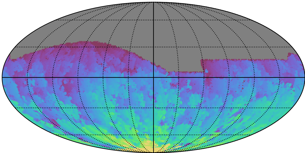
too_100_4v3.4_10yrs All sky g band: Max HA
