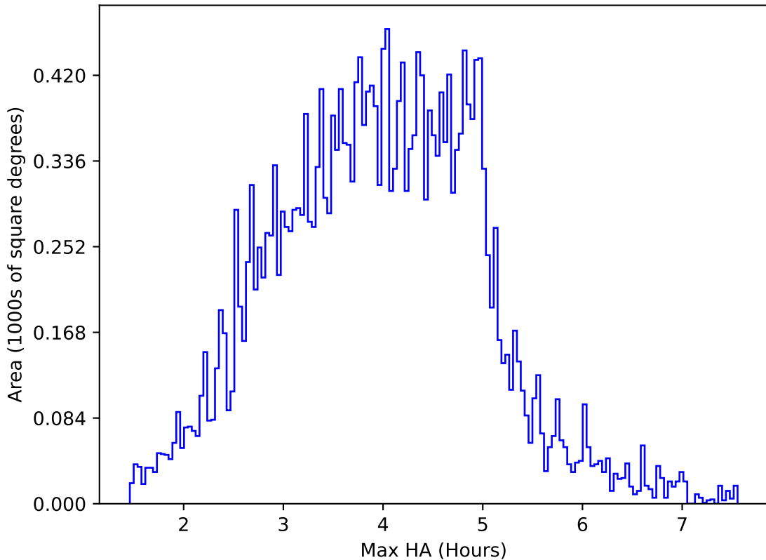
too_100_4v3.4_10yrs All sky g band: Max HA
