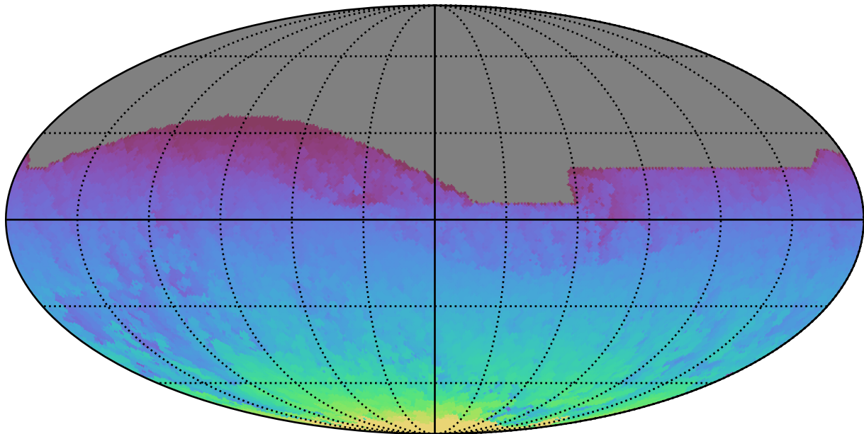
too_100_4v3.4_10yrs All sky all bands: Max HA
