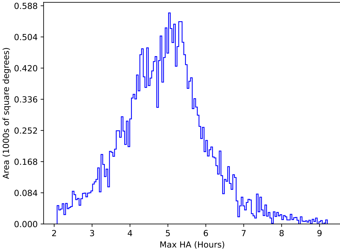
too_100_4v3.4_10yrs All sky all bands: Max HA
