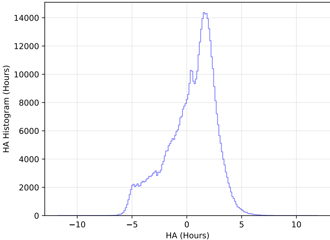
too_100_4v3.4_10yrs WFD r band: HA Histogram
