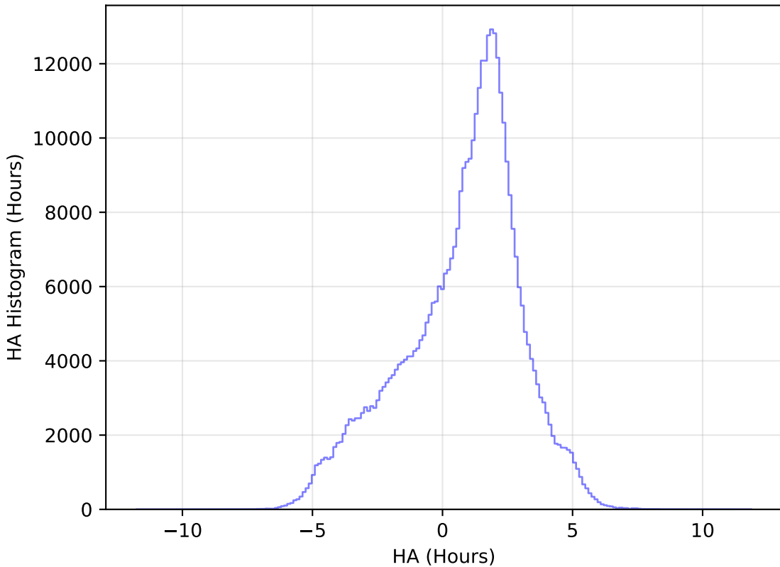
too_100_4v3.4_10yrs All sky z band: HA Histogram
