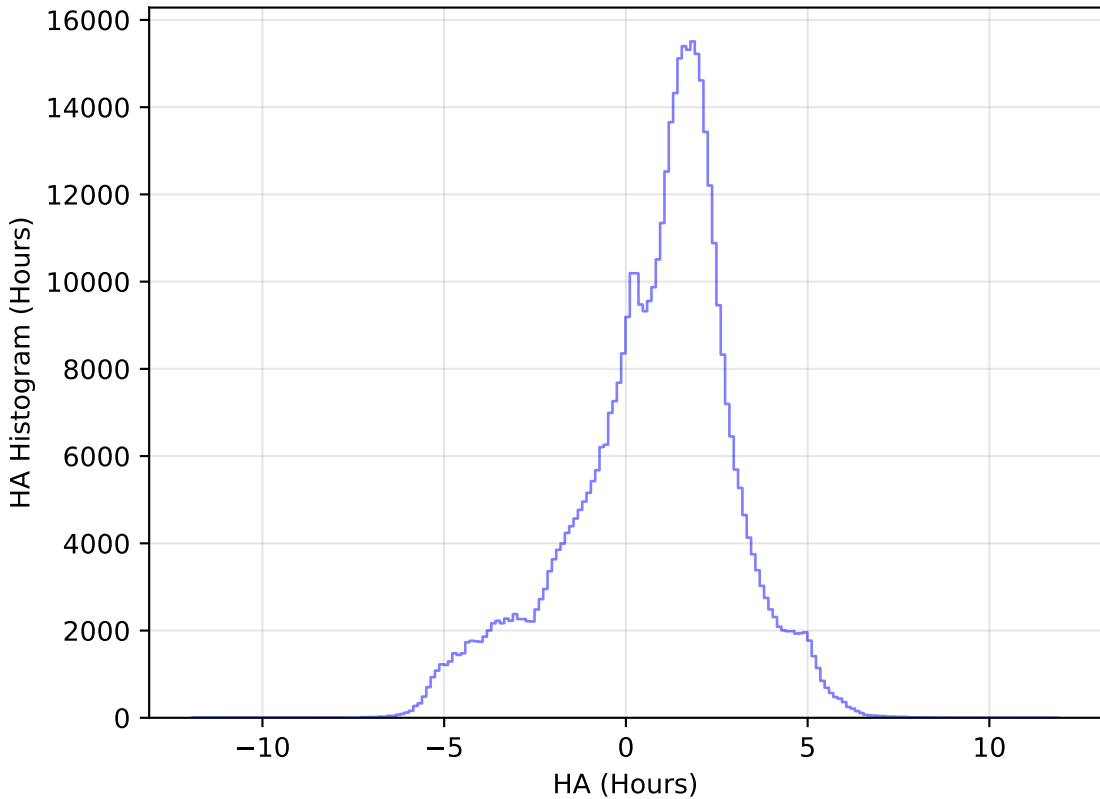
too_100_4v3.4_10yrs All sky i band: HA Histogram
