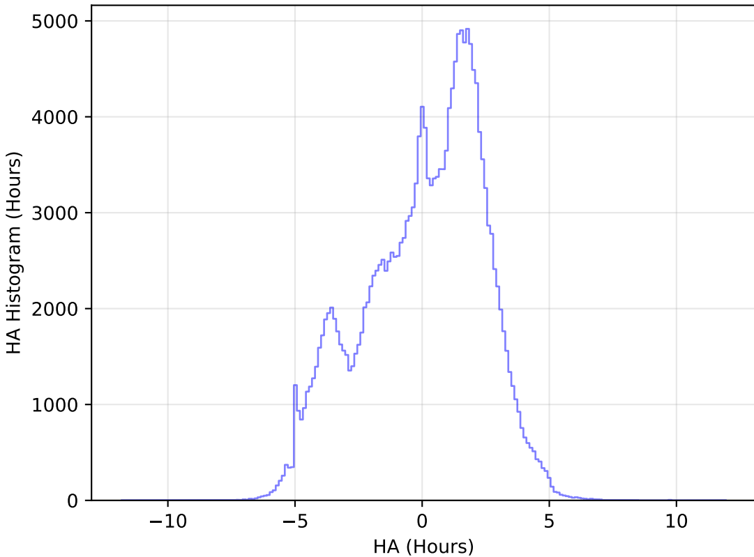
too_100_4v3.4_10yrs All sky g band: HA Histogram
