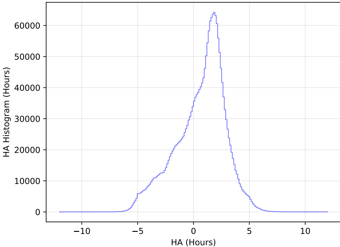
too_100_4v3.4_10yrs All sky all bands: HA Histogram
