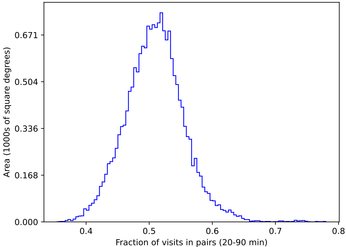
too_100_4v3.4_10yrs gri WFD: Fraction of visits in pairs (20-90 min)
