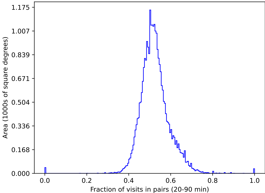
too_100_4v3.4_10yrs gri All sky: Fraction of visits in pairs (20-90 min)
