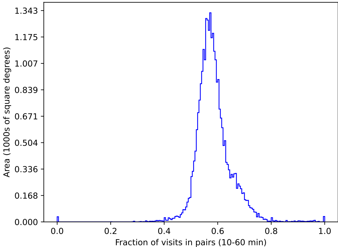
too_100_4v3.4_10yrs gri All sky: Fraction of visits in pairs (10-60 min)
