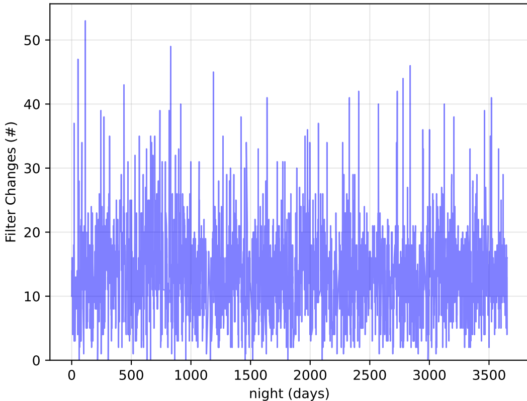
too_100_4v3.4_10yrs Per Night: Filter Changes
