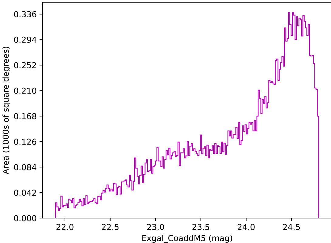
too_100_4v3.4_10yrs Yr 3-4 z band: Exgal_CoaddM5
