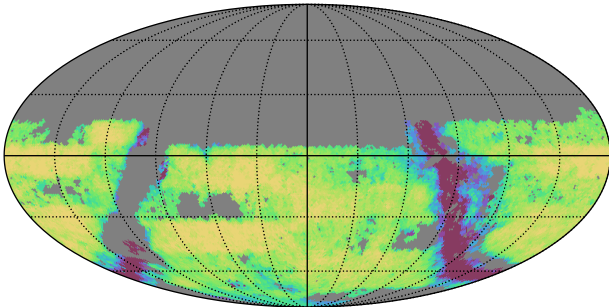
too_100_4v3.4_10yrs Yr 3-4 u band: Exgal_CoaddM5
