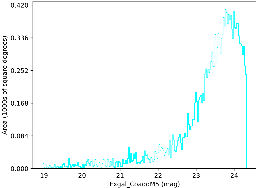
too_100_4v3.4_10yrs Yr 3-4 u band: Exgal_CoaddM5
