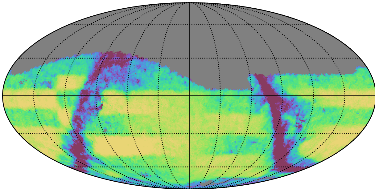
too_100_4v3.4_10yrs Yr 3-4 r band: Exgal_CoaddM5
