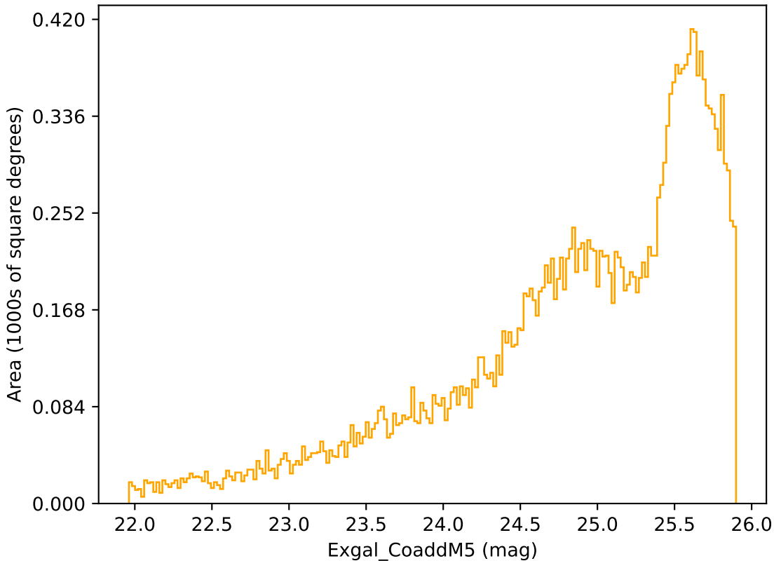
too_100_4v3.4_10yrs Yr 3-4 r band: Exgal_CoaddM5
