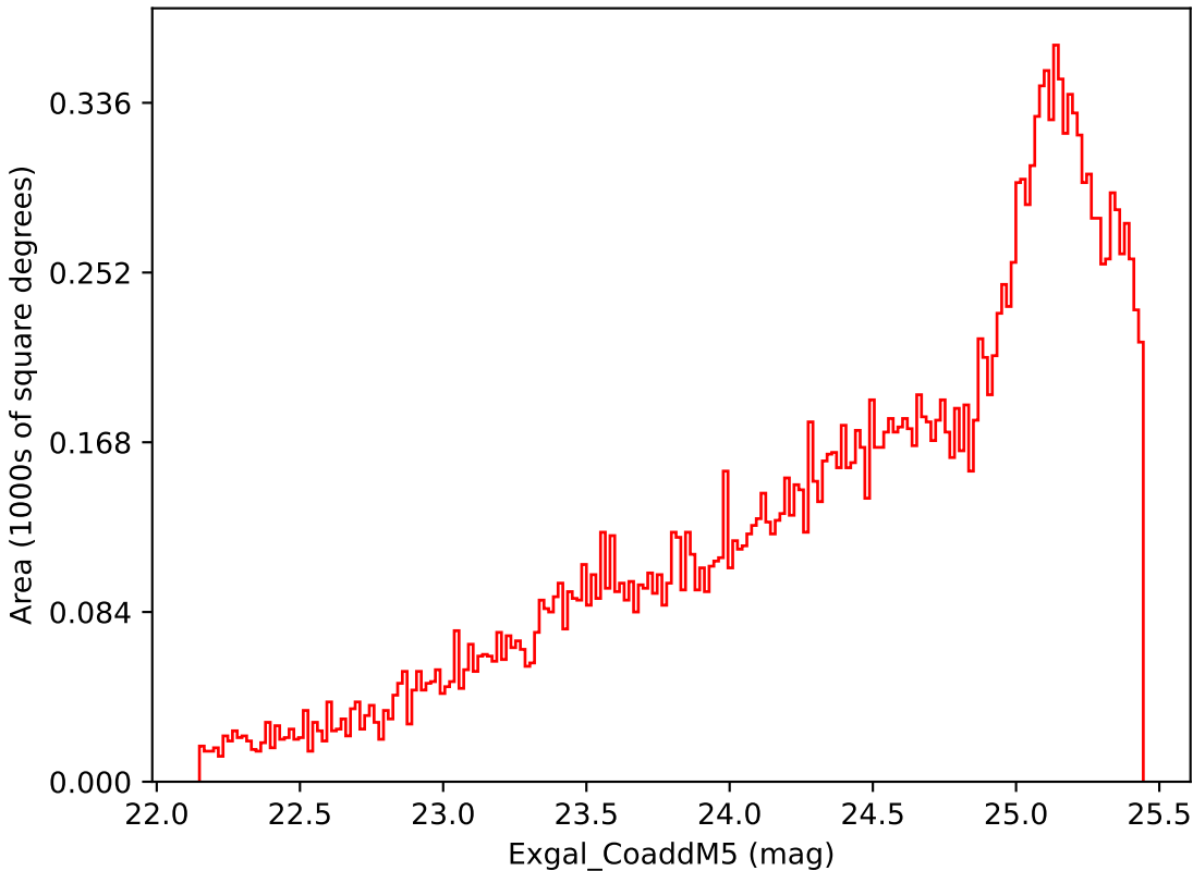
too_100_4v3.4_10yrs Yr 3-4 i band: Exgal_CoaddM5
