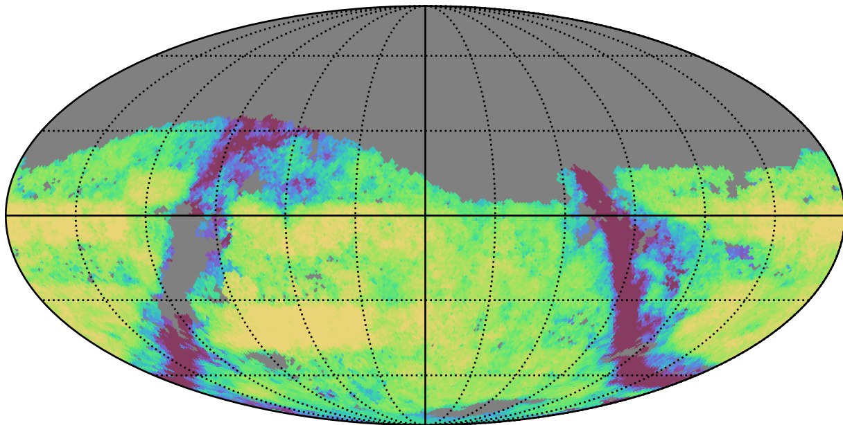
too_100_4v3.4_10yrs Yr 3-4 g band: Exgal_CoaddM5
