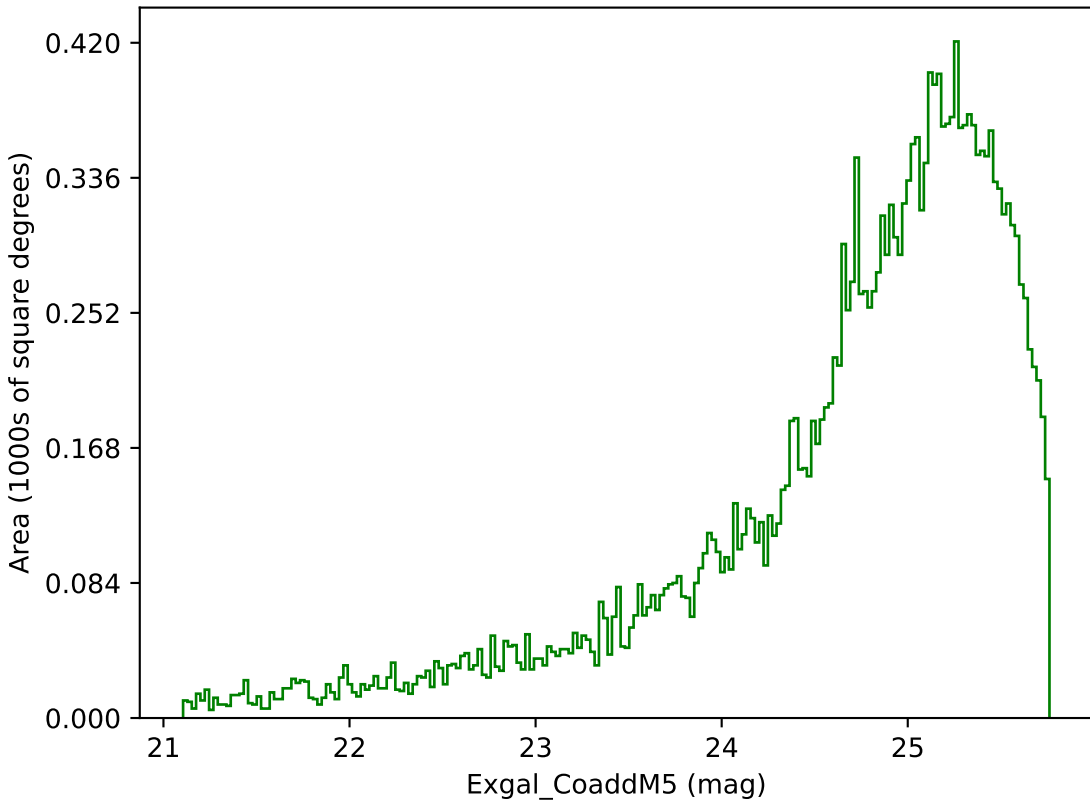
too_100_4v3.4_10yrs Yr 3-4 g band: Exgal_CoaddM5
