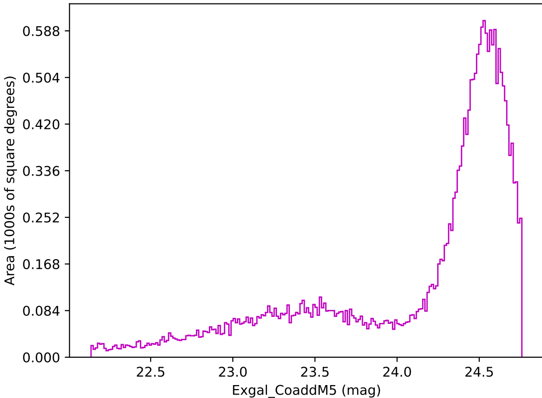
too_100_4v3.4_10yrs Yr 1 z band: Exgal_CoaddM5
