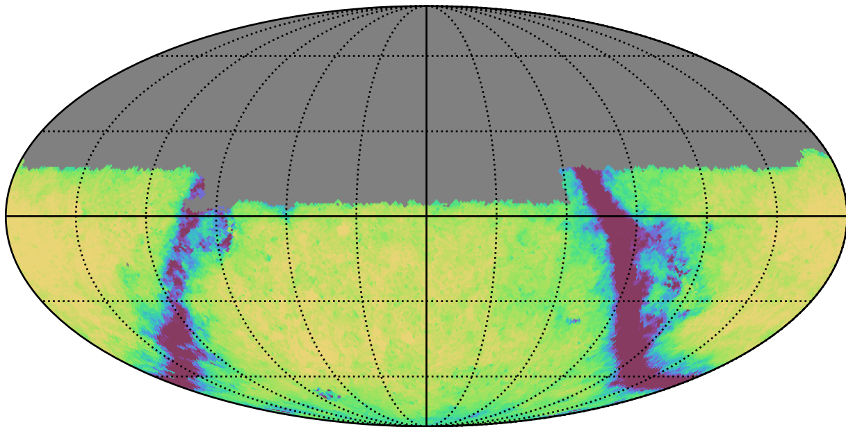
too_100_4v3.4_10yrs Yr 1 u band: Exgal_CoaddM5
