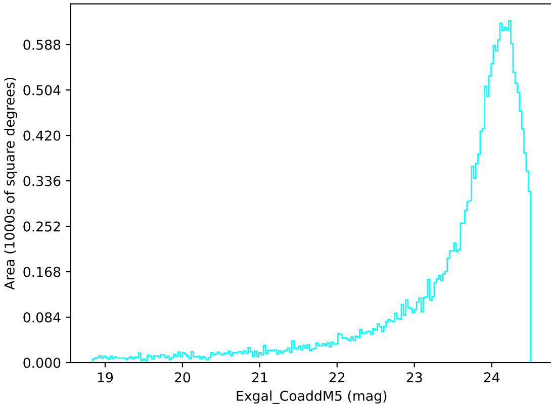
too_100_4v3.4_10yrs Yr 1 u band: Exgal_CoaddM5
