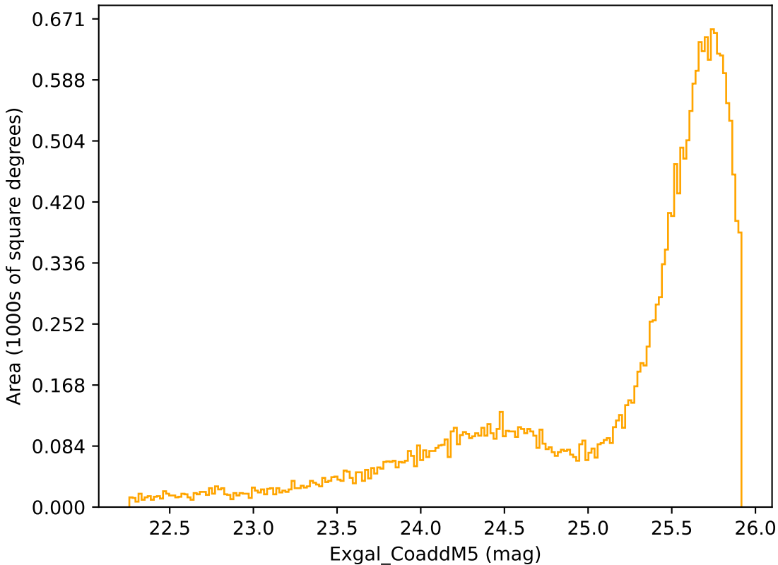
too_100_4v3.4_10yrs Yr 1 r band: Exgal_CoaddM5
