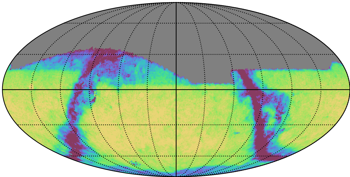
too_100_4v3.4_10yrs Yr 1 i band: Exgal_CoaddM5
