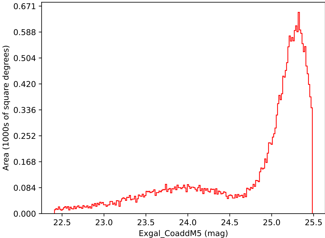
too_100_4v3.4_10yrs Yr 1 i band: Exgal_CoaddM5
