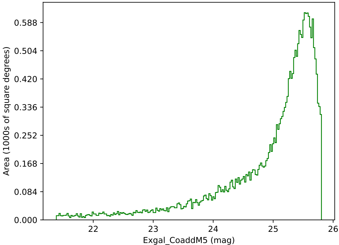
too_100_4v3.4_10yrs Yr 1 g band: Exgal_CoaddM5
