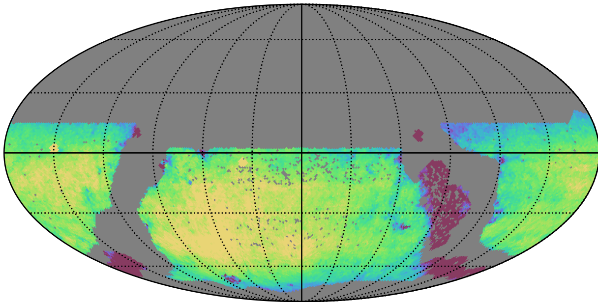
too_100_4v3.4_10yrs WFD z band: Exgal_CoaddM5
