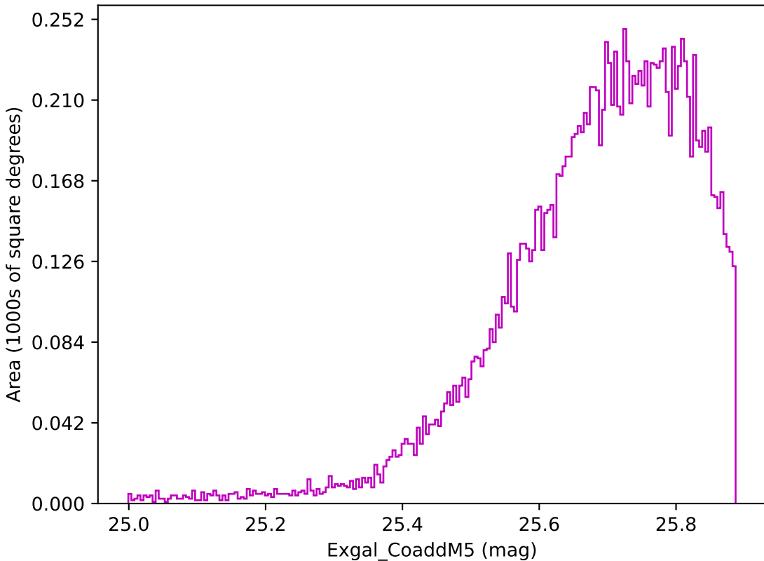
too_100_4v3.4_10yrs WFD z band: Exgal_CoaddM5
