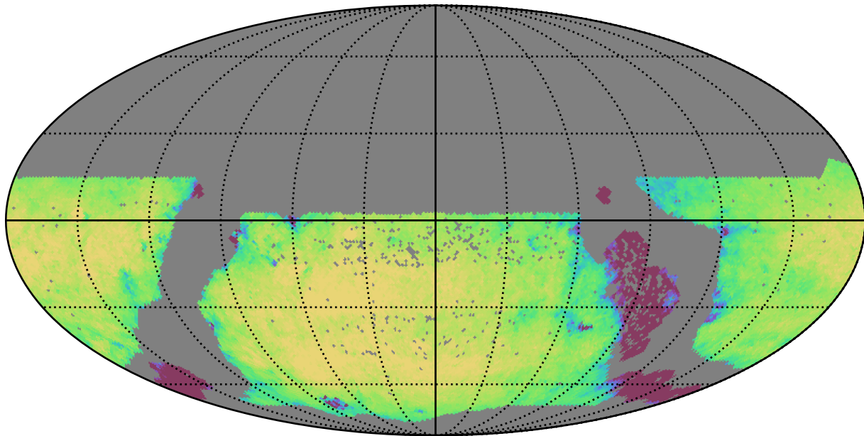
too_100_4v3.4_10yrs WFD u band: Exgal_CoaddM5
