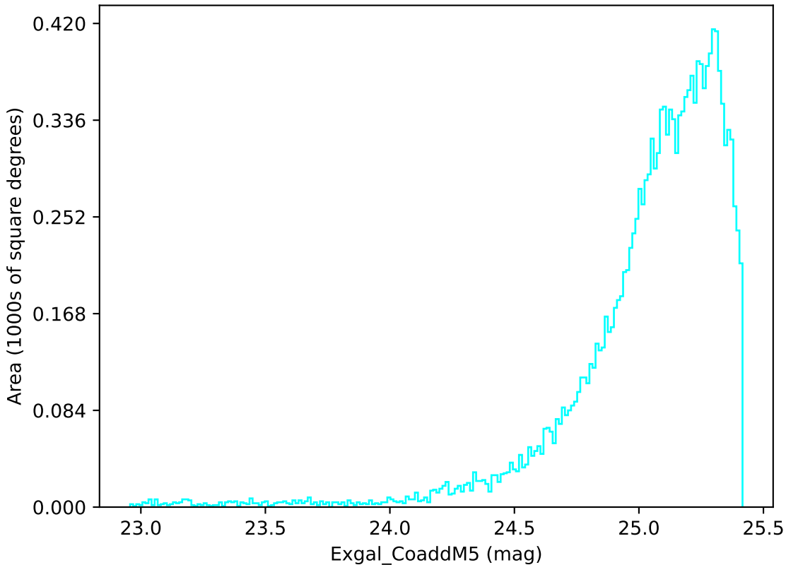
too_100_4v3.4_10yrs WFD u band: Exgal_CoaddM5
