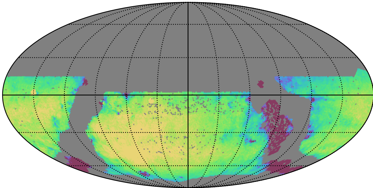
too_100_4v3.4_10yrs WFD r band: Exgal_CoaddM5
