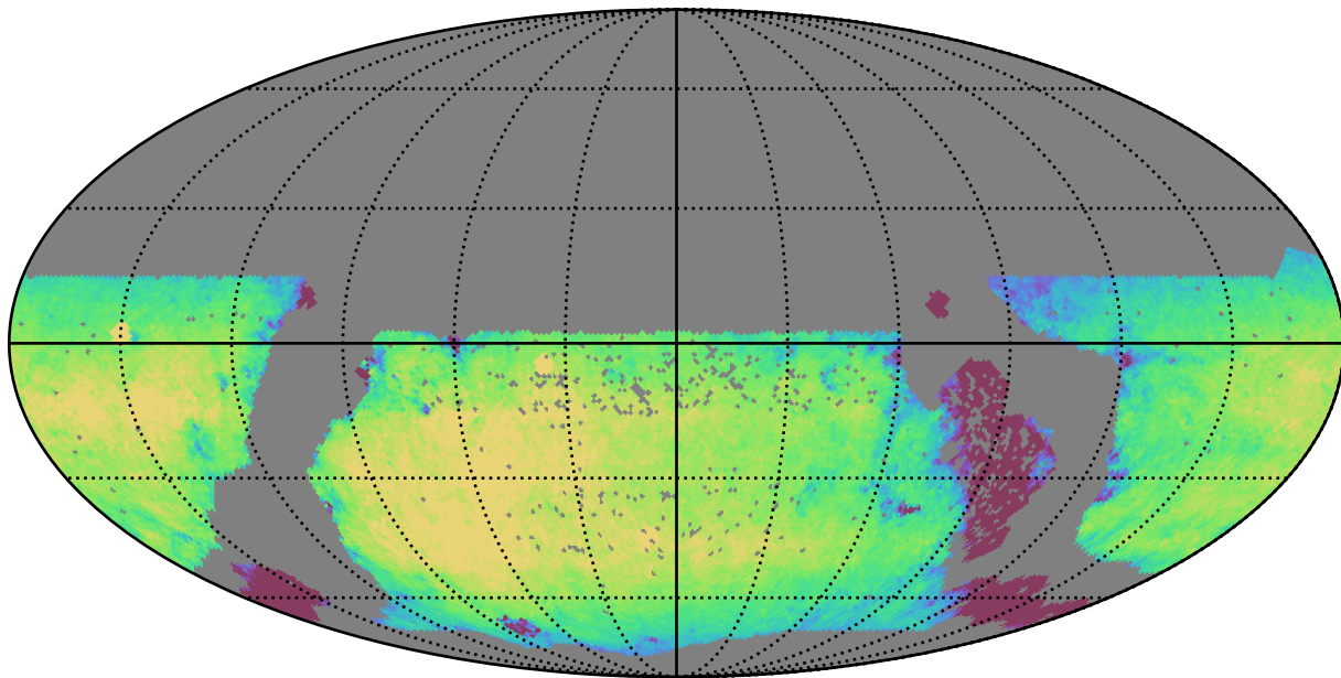
too_100_4v3.4_10yrs WFD i band: Exgal_CoaddM5
