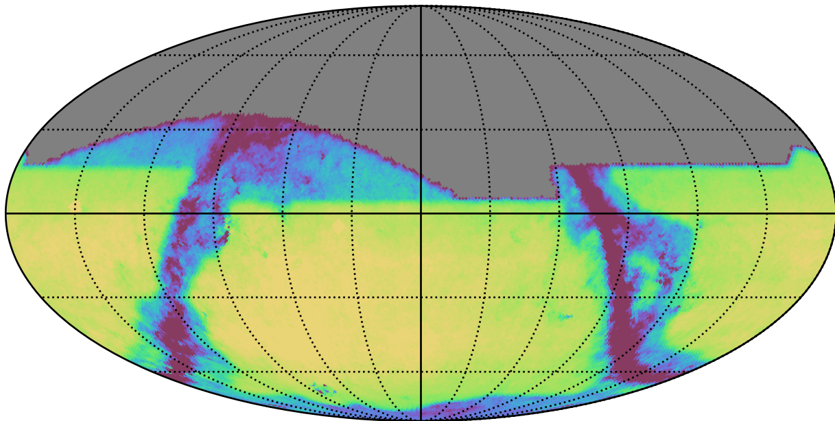
too_100_4v3.4_10yrs All sky z band: Exgal_CoaddM5
