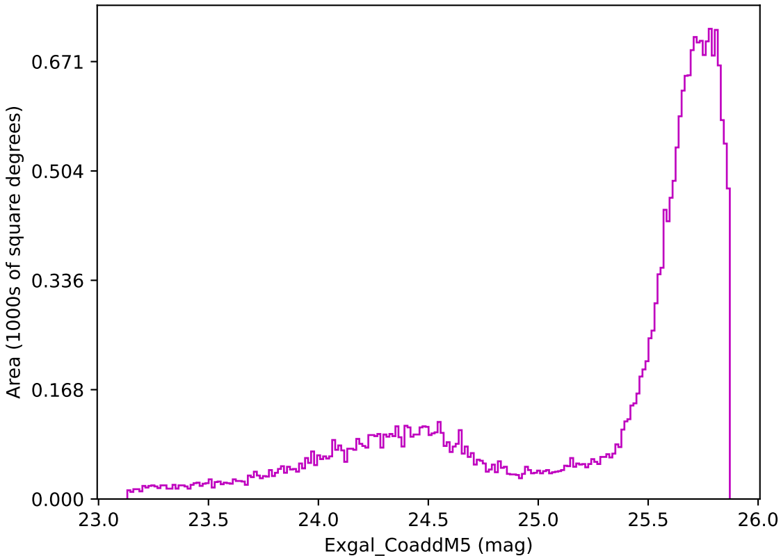
too_100_4v3.4_10yrs All sky z band: Exgal_CoaddM5
