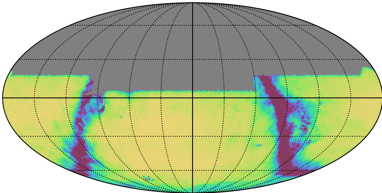
too_100_4v3.4_10yrs All sky u band: Exgal_CoaddM5
