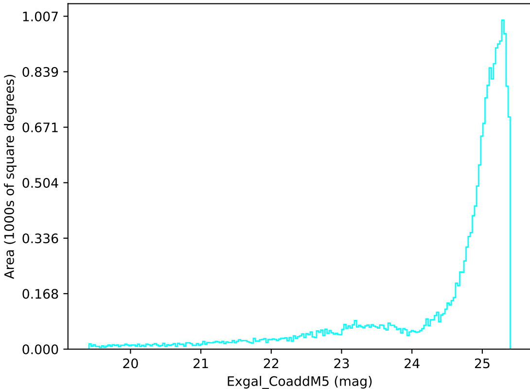
too_100_4v3.4_10yrs All sky u band: Exgal_CoaddM5
