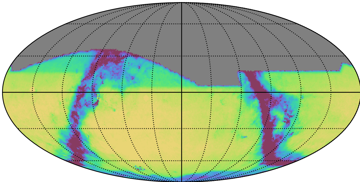
too_100_4v3.4_10yrs All sky r band: Exgal_CoaddM5
