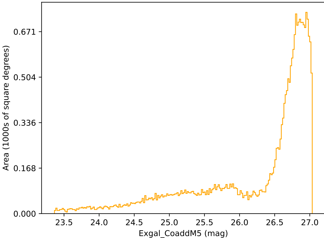
too_100_4v3.4_10yrs All sky r band: Exgal_CoaddM5
