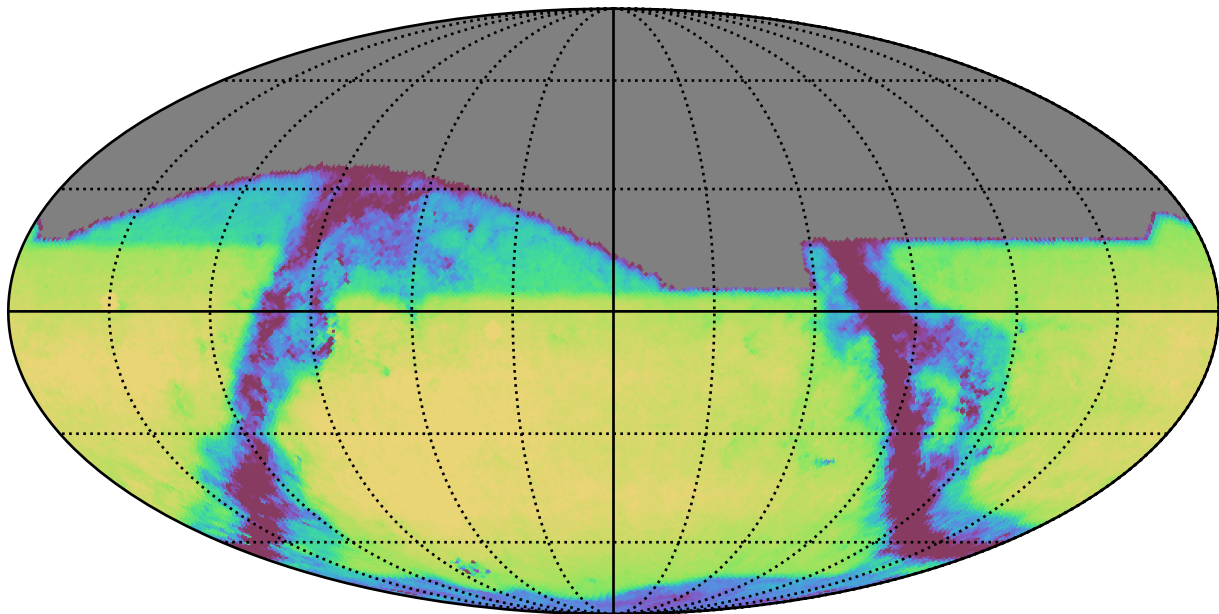
too_100_4v3.4_10yrs All sky i band: Exgal_CoaddM5
