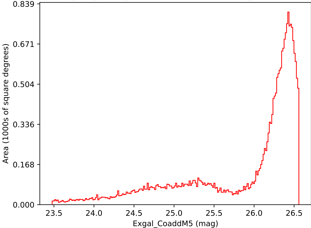
too_100_4v3.4_10yrs All sky i band: Exgal_CoaddM5
