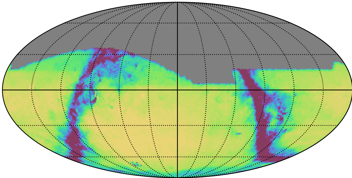
too_100_4v3.4_10yrs All sky g band: Exgal_CoaddM5
