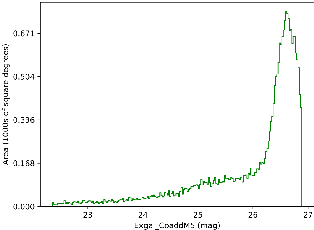
too_100_4v3.4_10yrs All sky g band: Exgal_CoaddM5
