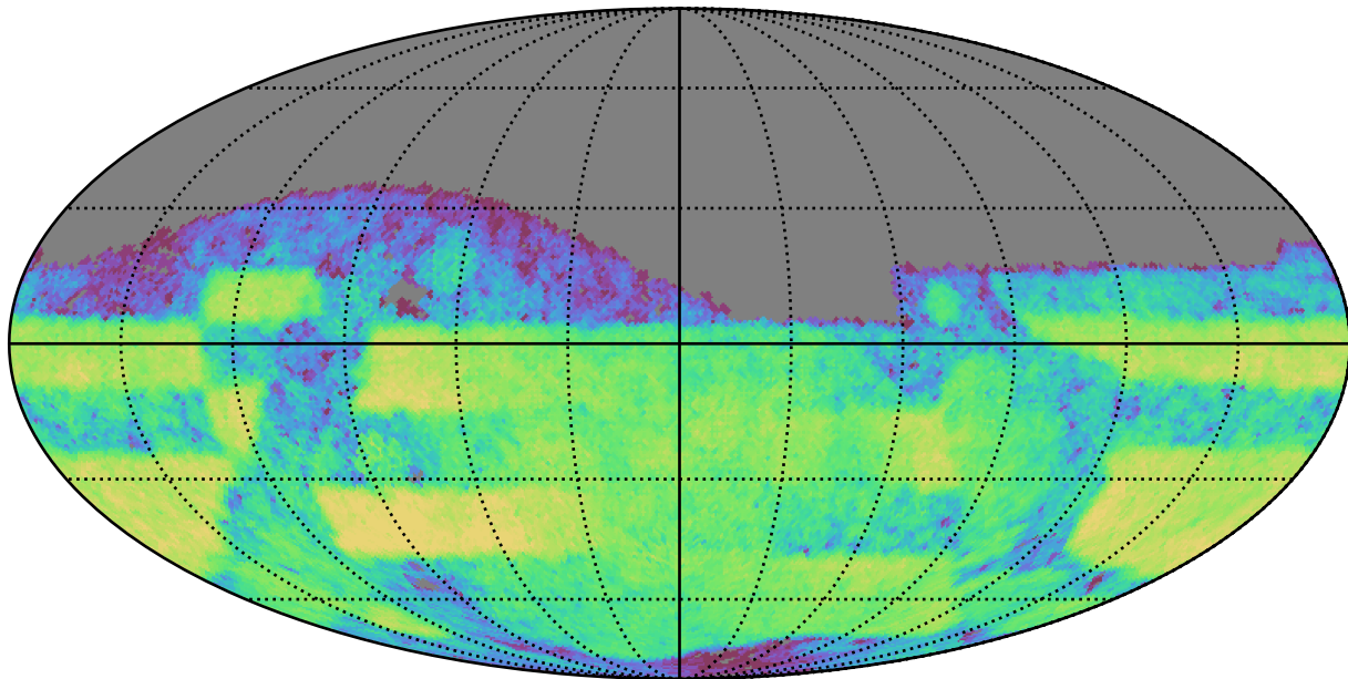
too_100_4v3.4_10yrs Yr 3-4 z band: CoaddM5
