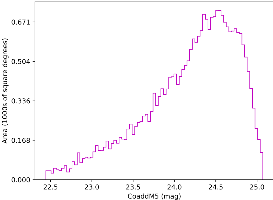
too_100_4v3.4_10yrs Yr 3-4 z band: CoaddM5
